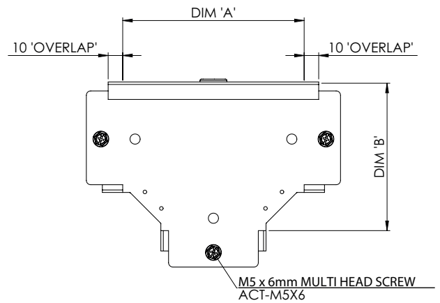
ASB - SCREWBUSH
