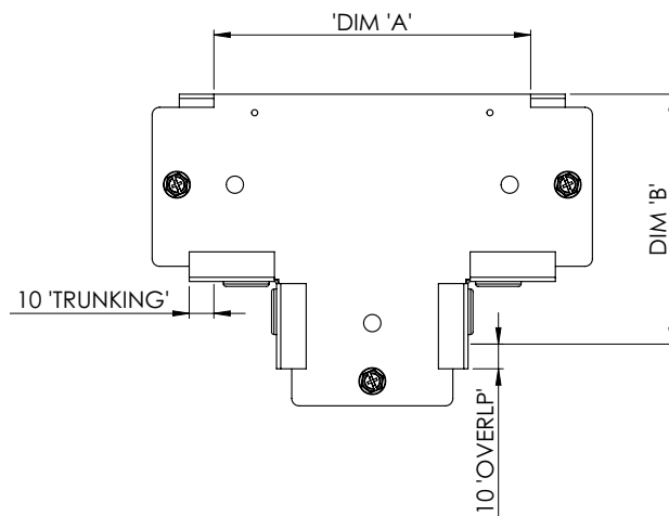
ASB - SCREWBUSH
